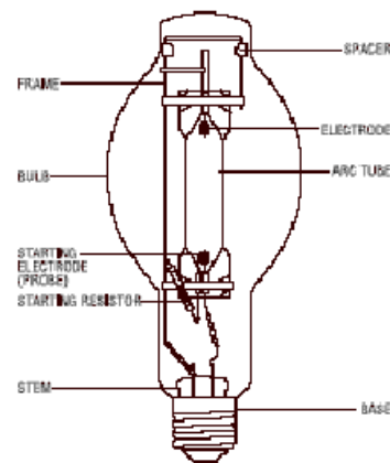
FIGURE 4-7 Mercury vapor lamp composition. Courtesy of OSRAM SYLVANIA, Inc.
